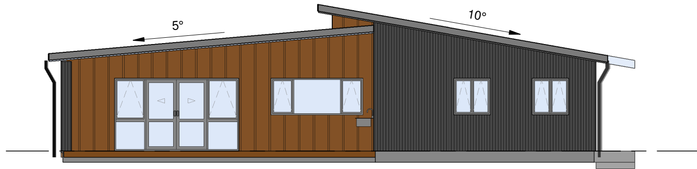
3 West Elevation A05 Scale 1 : 100
